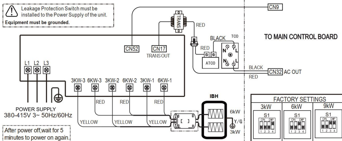
Figure1: 9kW IBH(Three step control)
