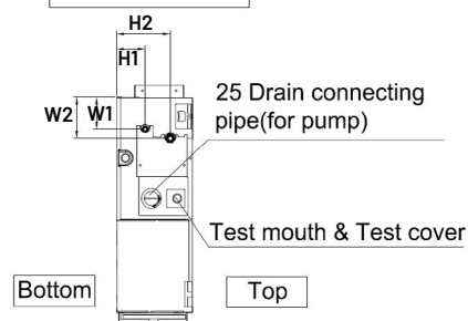
Pipe side view
